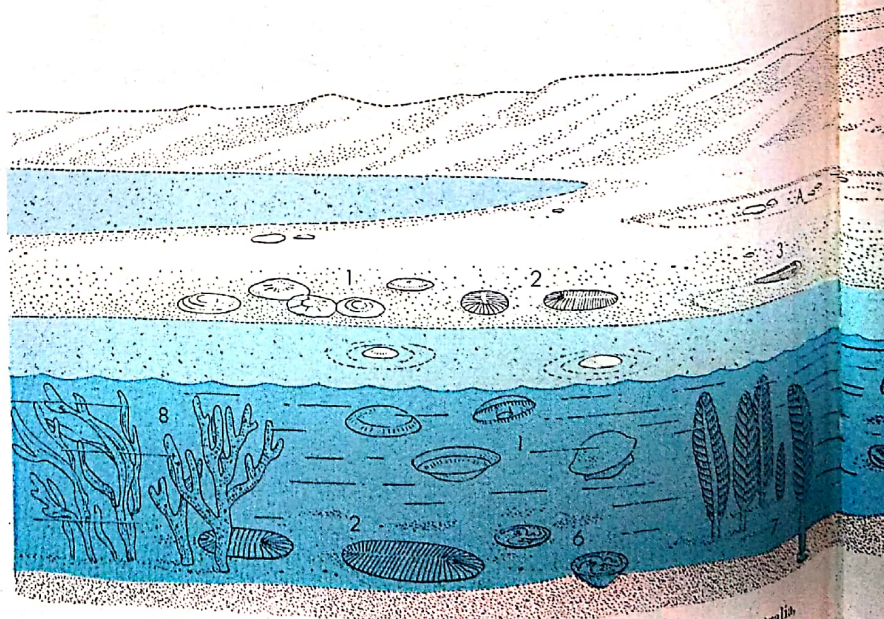
PRE-CAMBRIAN SEASHORE AREA, reconstructed from fossils found in South Australia. supported several types of animal. Some are shown stranded in dried-up mudholes (4) and on sand of beach, where they were fossilized. Others appear (lower left) in sand and
