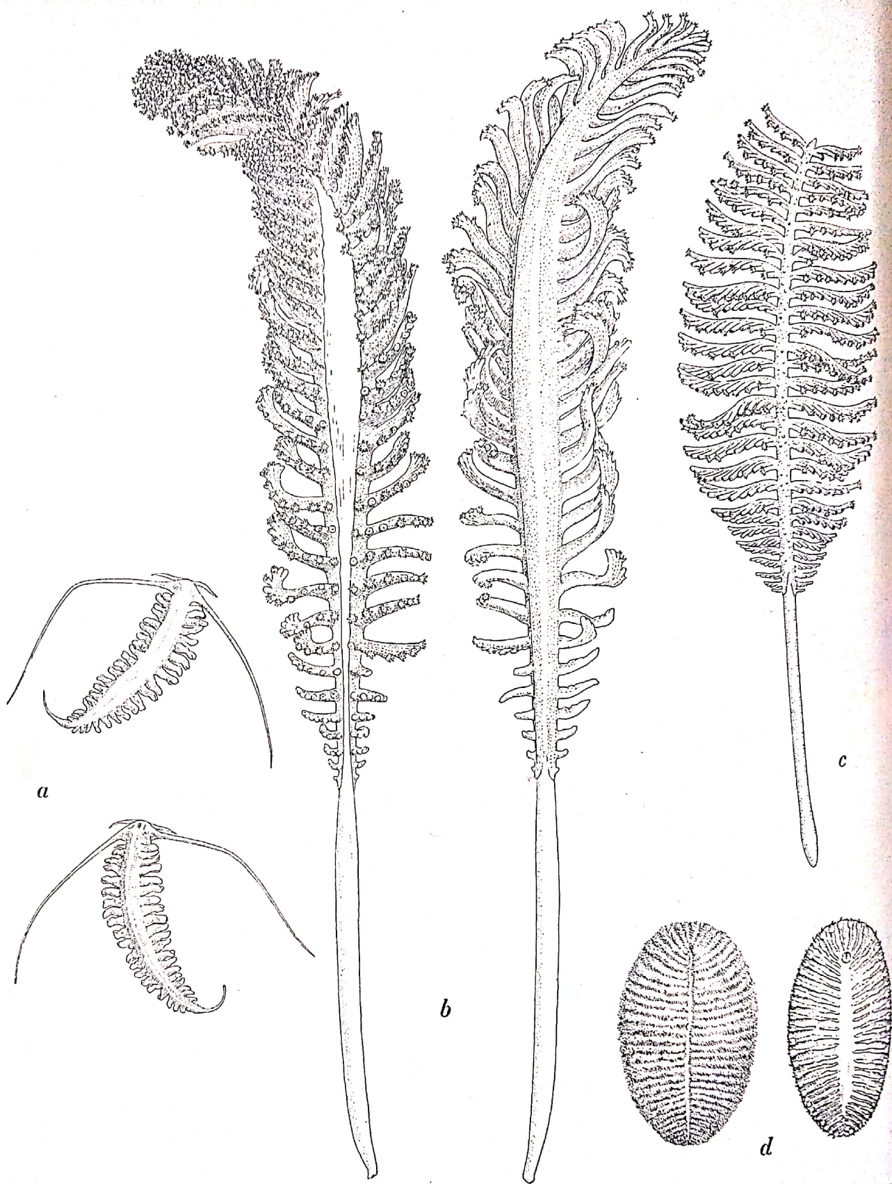
Pennatula rubra (b), shown front and back, and Pennatula aculeata (c); and the worm Spinther citrinus (d), which looks like the many specimens of Dickinsonia in the Pre-Cambrian rocks.
