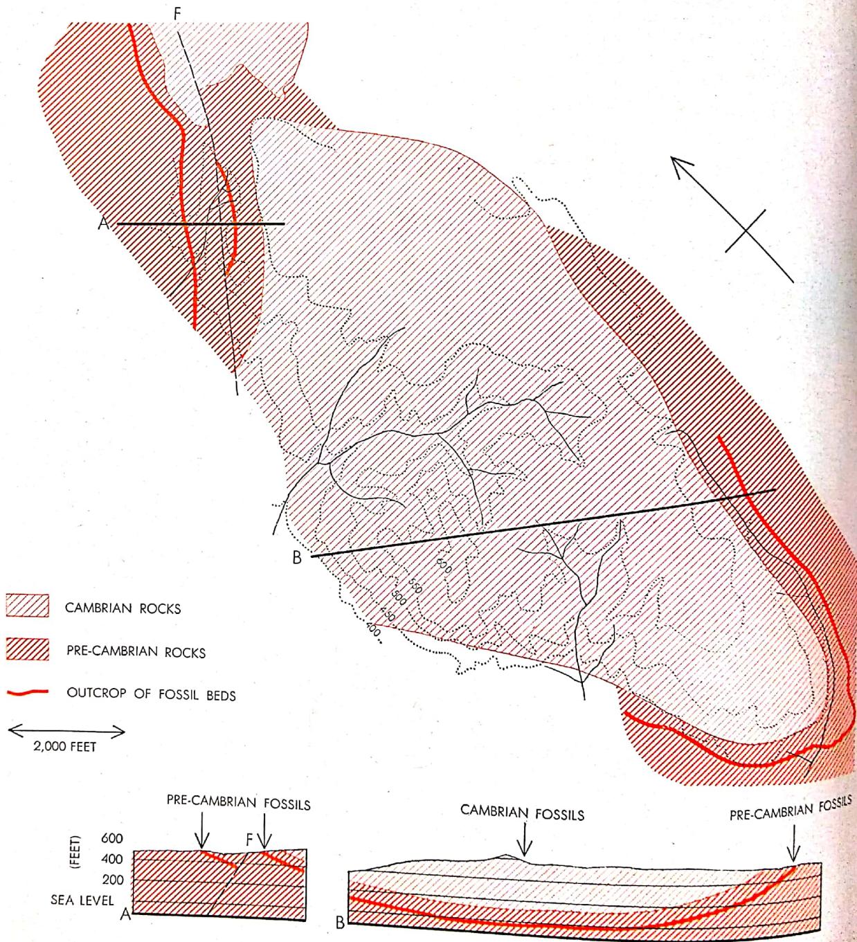
MAP AND CROSS SECTIONS OF SITE where fossils are found show relative positions of Cambrian and Pre-Cambrian rocks. Lines A and B indicate locations of cross sections A and B (below map). Broken line F is a fault that has caused part of Pre-Cambrian fossil
