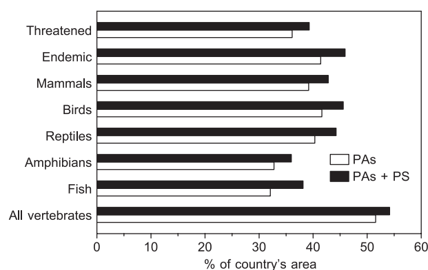
Figure 5 Percentage of the total country area required to achieve the conservation targets when the current reserve network (PAs; open bars), and the current reserve network and proposed priority sites (PAs + PS; solid bars) are included in the analysis.
